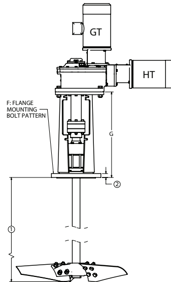
GT/HT N Spacer Spool
