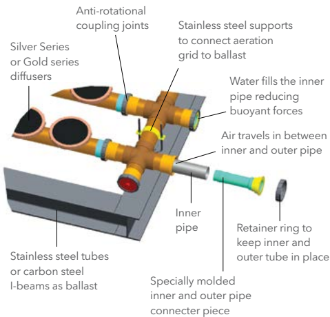
Tube-in-tube design
