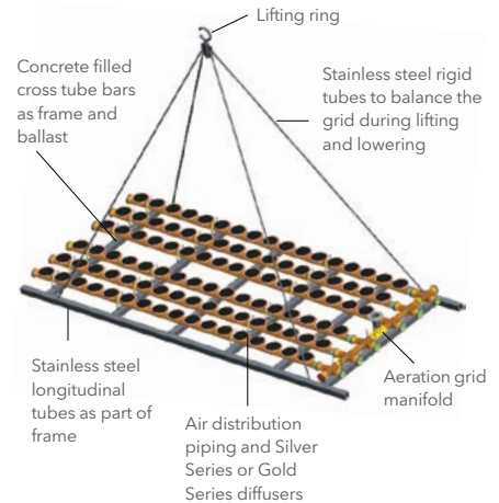
Lifting Arrangement Option 2
