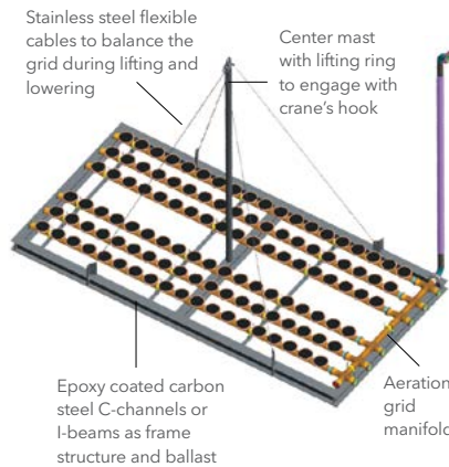
Lifting Arrangement Option 1
