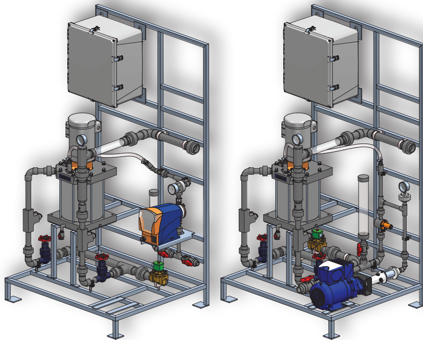
Diaphragm Metering Pump Systems
